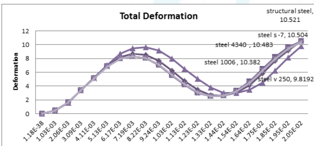
Figure 6: Time vs. Total Deformation
