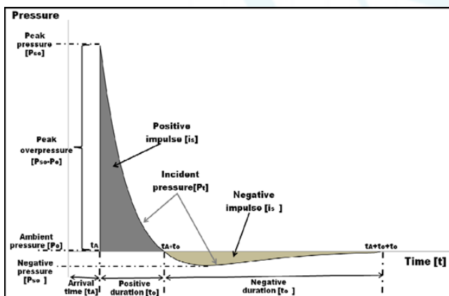
Figure 3: Ideal blast wave's pressure time history
