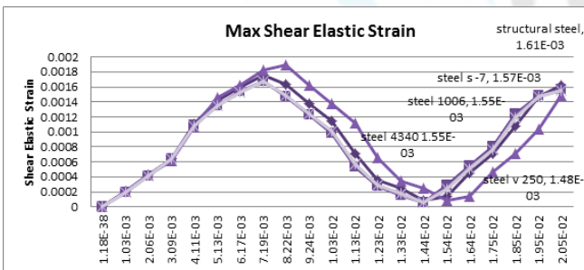
Figure 7: Time vs Max Shear Elastic Strain
