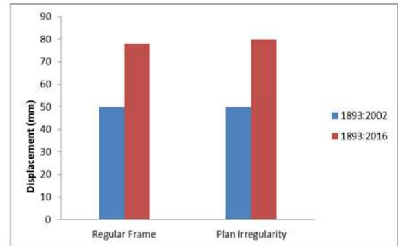
Figure 7: Maximum lateral displacement in mm in X direction
