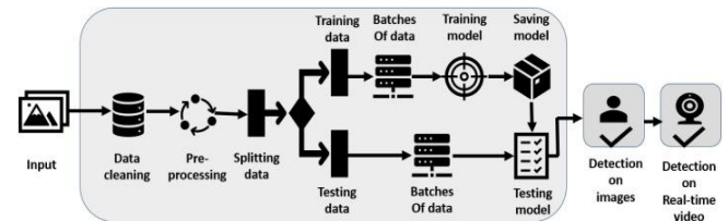
Figure 2: CNN Architecture
