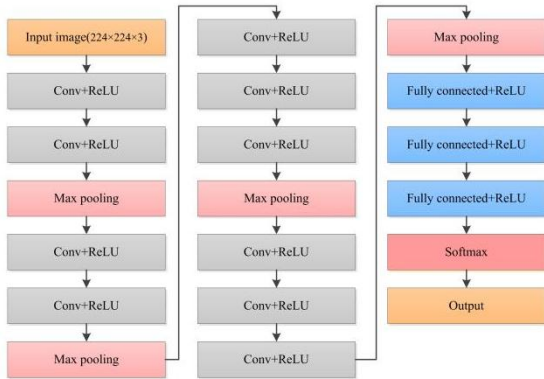
Figure 2.3-1: VGG-16 structure
