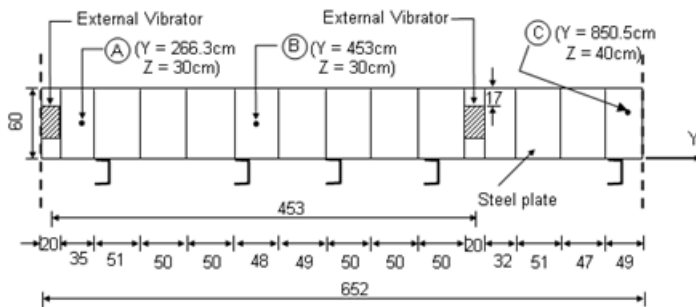
Figure 7: Detail of the measuring face (column element)
