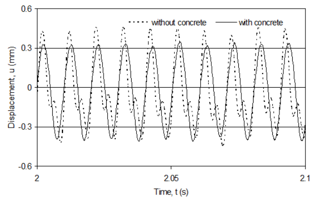
Figure 8: Change of measuring point A with respect to time
