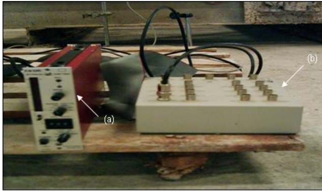
Figure 1: Dynamic Strain Meter, DA-32D type (Tokyo Sokki Kenkyujo Co., Ltd.)
