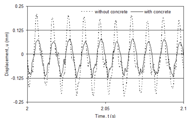
Figure 10: Change of measuring point C with respect to time
