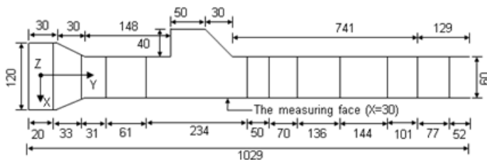
Figure 6: Plan view of the mold of the column element ( h = 60 cm)
