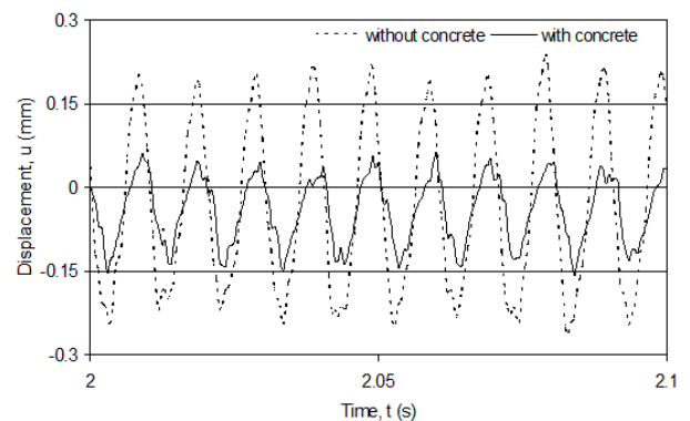
Figure 9: Change of measuring point B with respect to time
