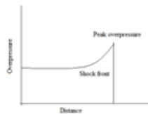
Figure 2: Formation of shock front
