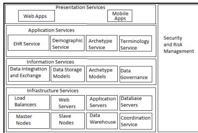
Figure 4: Architecture of CHISTAR
