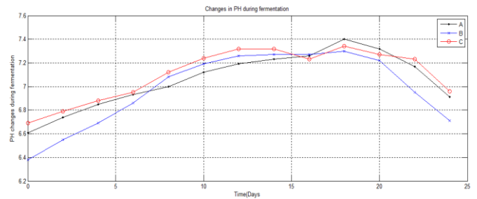
Figure 3: PH changes during Fermentation, A-Poultry Droppings + Cassava Peelings +Water, B-Poultry Droppings +Beans waste + water, C-Cassava Peelings + Beans waste +water
