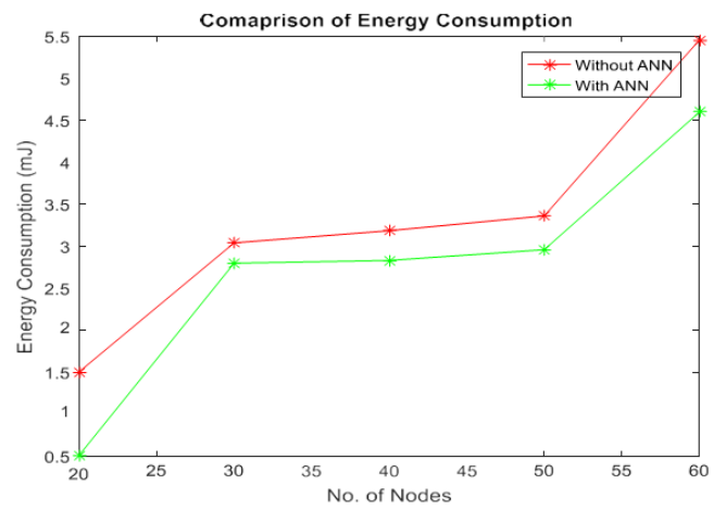
Figure 5.4: Energy Consumption
